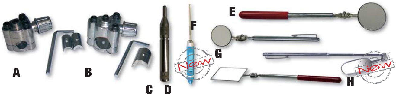
Bullet piercing valve, core remover and mirrors
